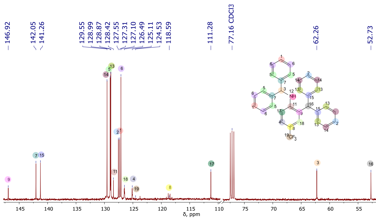
Figure S23. Selected area of 13 C NMR spectrum of compound 8 in CDCl 3 .
