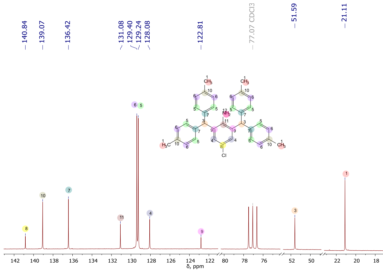
Figure S16. Selected area of 13 C NMR spectrum of compound 5 in CDCl 3 .
