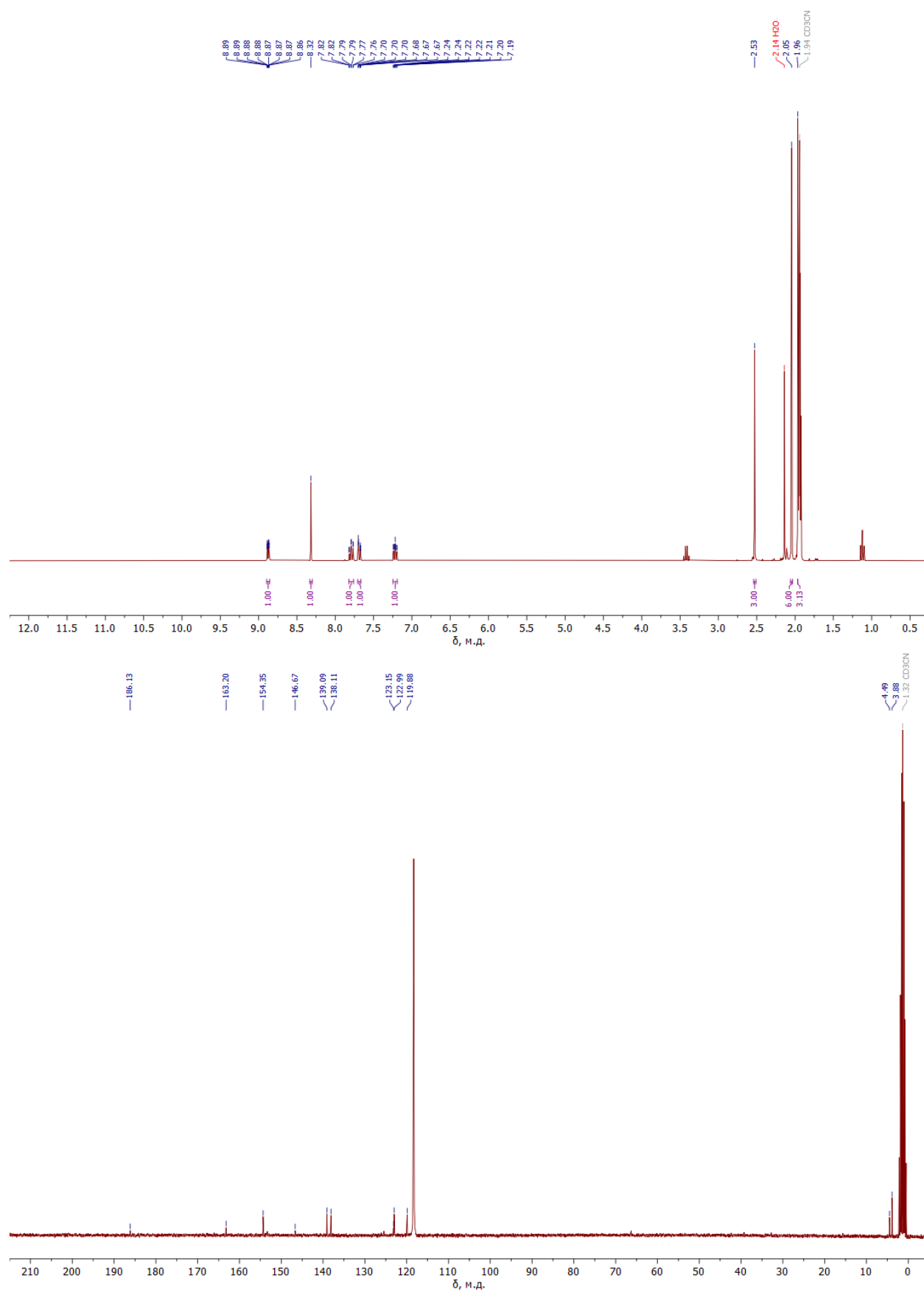
Fig. 5. ^1\text{H} and ^{13}\text{C} NMR spectra of 2e .
