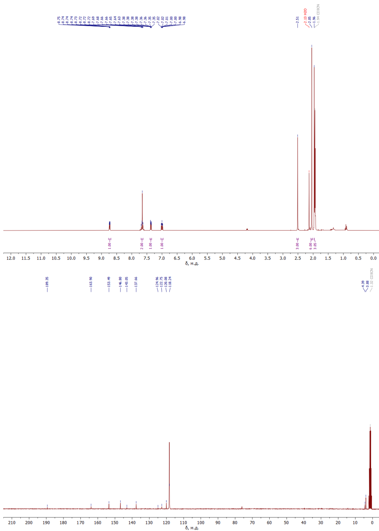
Fig. 4. ^1\text{H} and ^{13}\text{C} NMR spectra of 2d .
