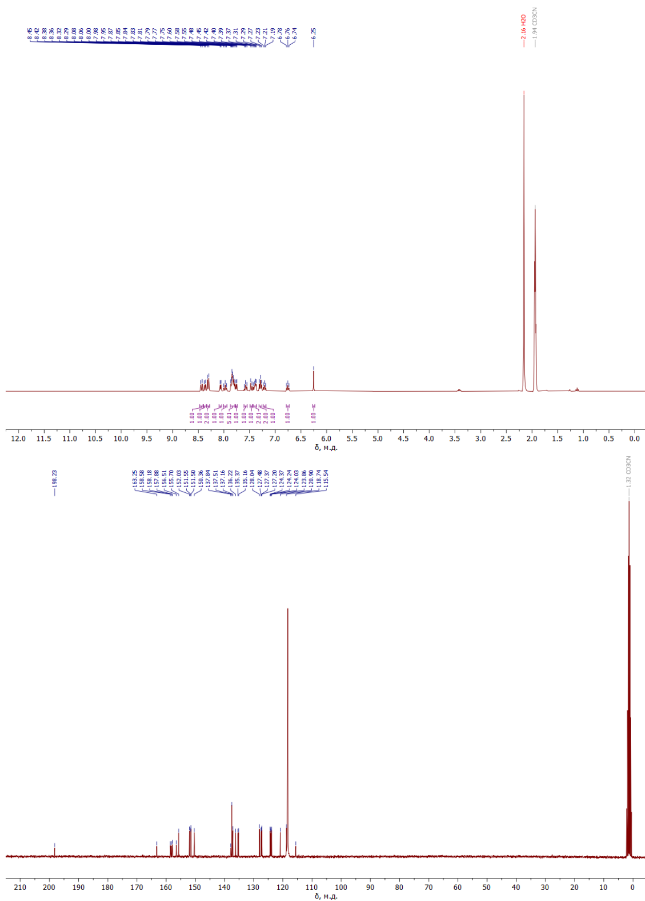
Fig. 9. ^1\text{H} and ^{13}\text{C} NMR spectra of 3c .
