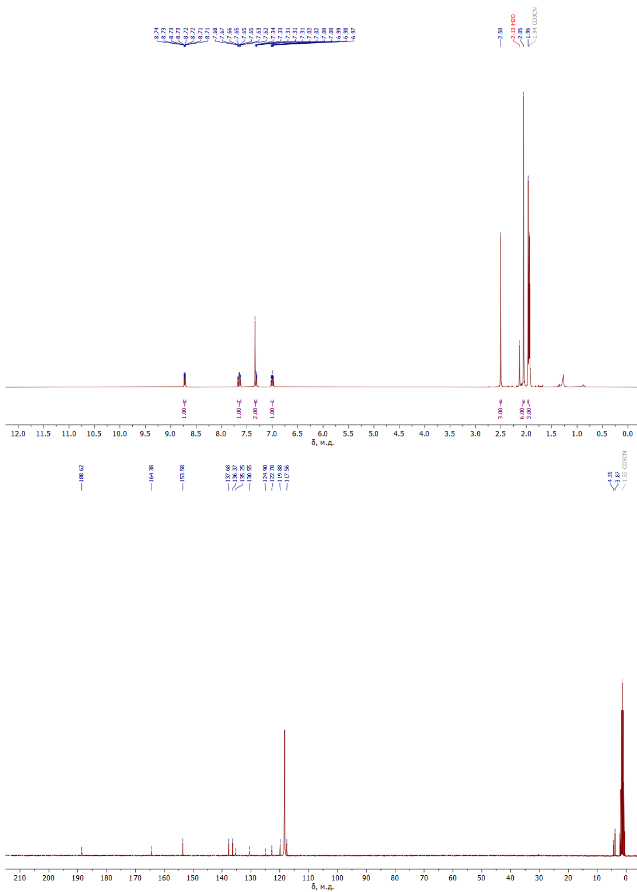
Fig. 2. ^1\text{H} and ^{13}\text{C} NMR spectra of 2b .
