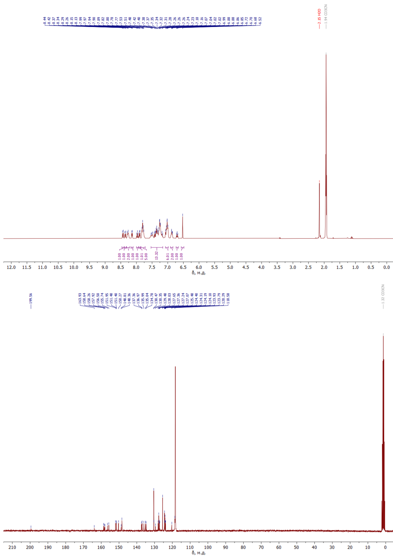
Fig. 12. ^1\text{H} and ^{13}\text{C} NMR spectra of 3f .
